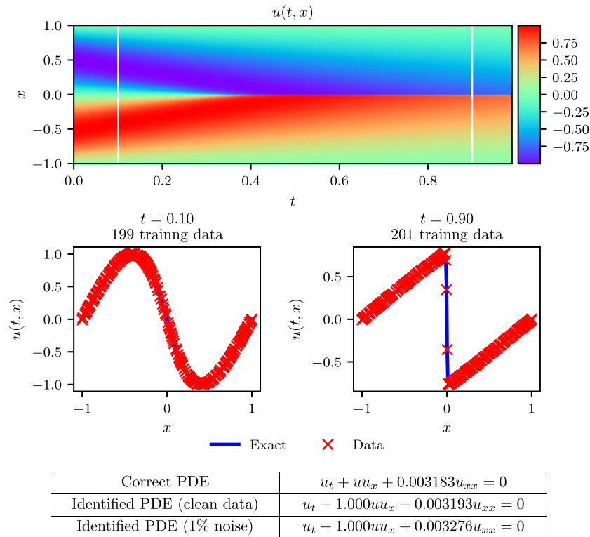
Fig. B.9. Burgers equation: Top: Solution u(t, x) along with the temporal locations of the two training snapshots. Middle: Training data and exact solution corresponding to the two temporal snapshots depicted by the dashed vertical lines in the top panel. Bottom: Correct partial differential equation along with the identified one obtained by learning \lambda_1, \lambda_2 .
