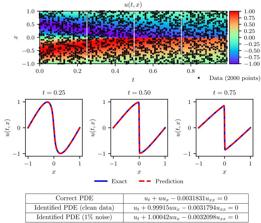
Fig. B.8. Burgers equation: Top: Predicted solution u(t, x) along with the training data. Middle: Comparison of the predicted and exact solutions corresponding to the three temporal snapshots depicted by the dashed vertical lines in the top panel. Bottom: Correct partial differential equation along with the identified one obtained by learning \lambda_1 and \lambda_2 .
